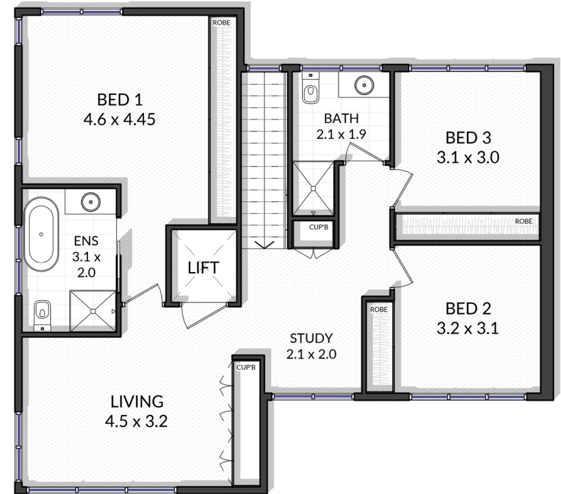
FIRST LEVEL FLOOR PLAN
