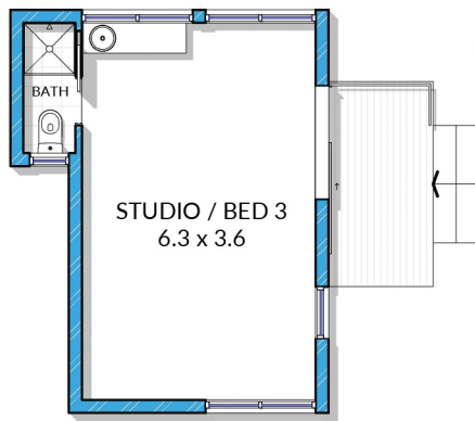
STUDIO FLOOR PLAN
