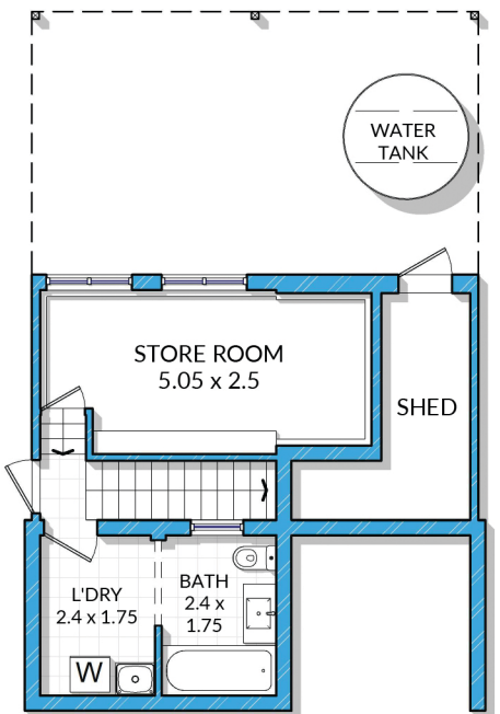
LOWER GROUND LEVEL FLOOR PLAN
