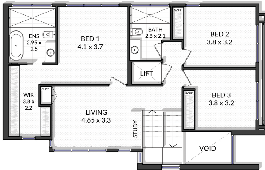
FIRST LEVEL FLOOR PLAN
